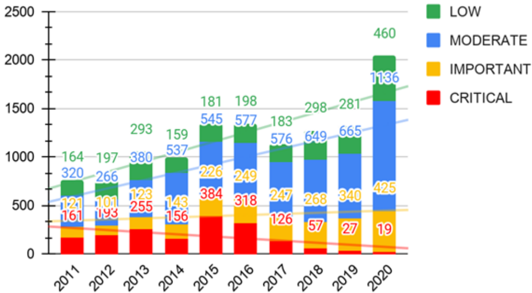
Figure 2: Report vulnerabilities
